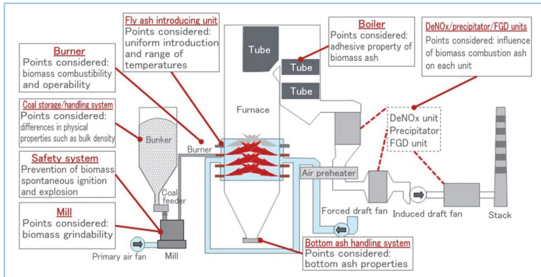
Figure 3 Conceptual diagram of power generation facility with boiler exclusively fired with pulverized biomass
