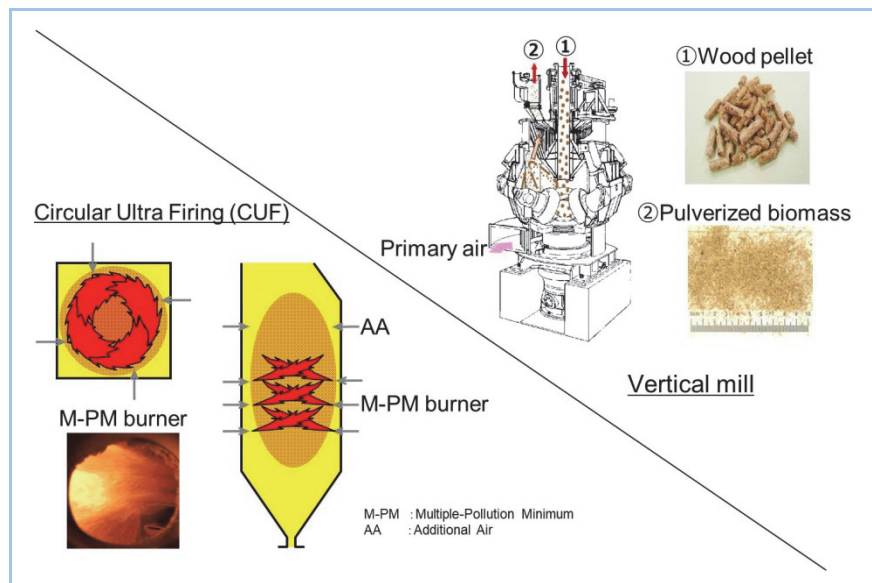
Figure 1 Pulverized biomass firing technology
