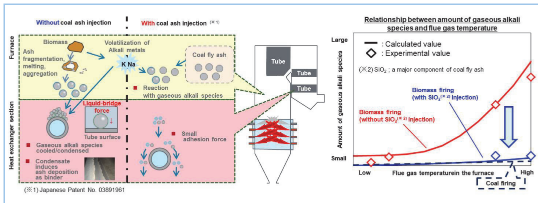
Figure 2 Ash deposition mechanism and effect of ash deposition prevention by coal ash introduction
