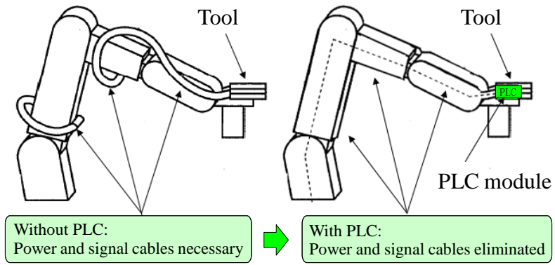
Fig. 1: Wiring reduction through application of PLC
