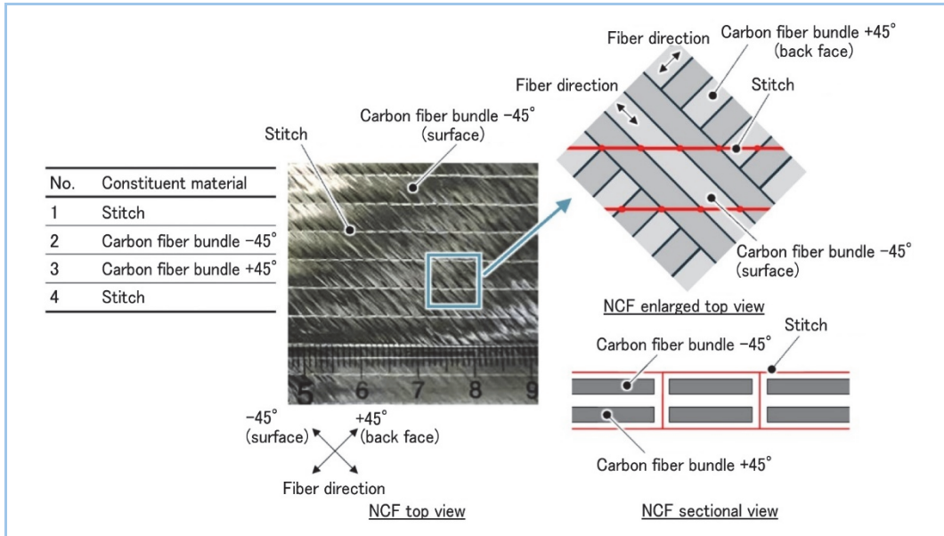
Figure 1 Targeted NCF configuration The material (NCF) discussed in this report is composed of the constituent materials listed in the table above. Two layers of carbon fiber bundles arranged in the directions of -45° and +45° are stitched together.
