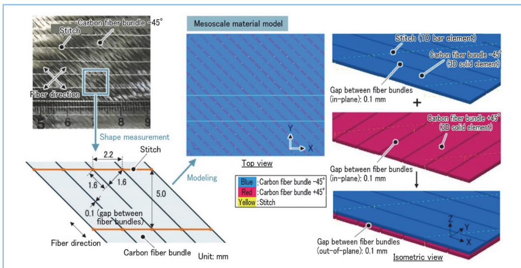
Figure 2 Mesoscale material model of NCF We measured the shape of the actual NCF and created mesoscale material model to match the actual NCF. The fiber bundles in the -45° and +45° directions were modeled by three-dimensional solid elements, and the stitches were modeled by one-dimensional bar elements.
