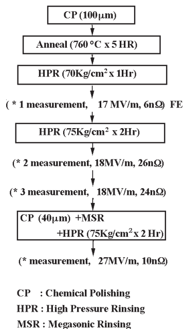
Fig.5 Surface treatment of the M-5 cavity (after repaired)
