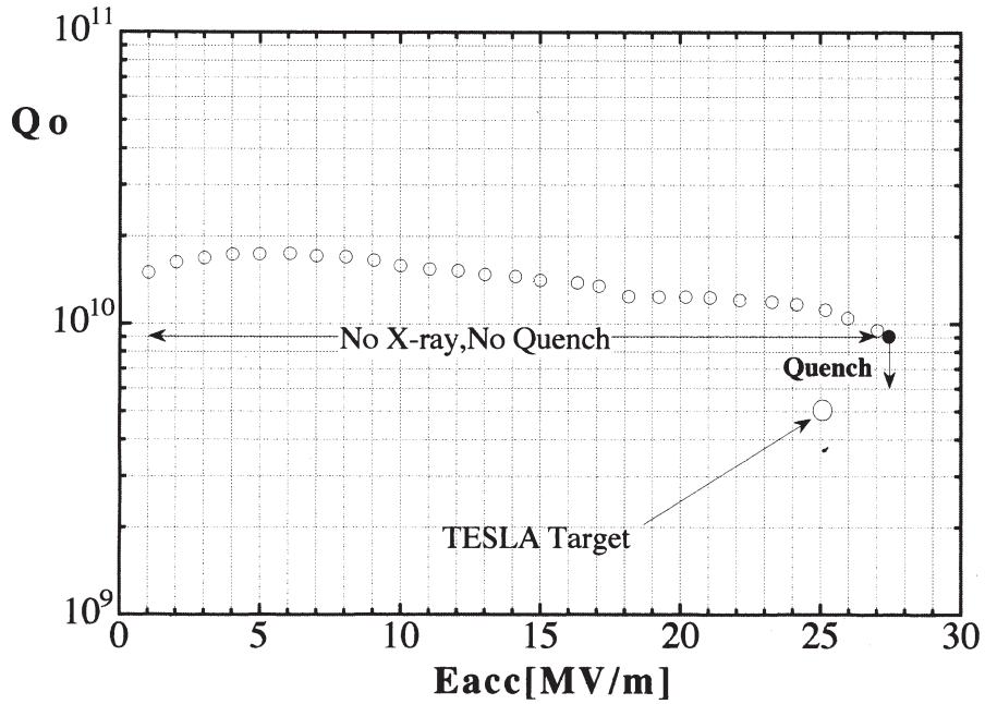
Fig.6 Q_0 - E_{acc} plots in the cold test of the M-5 cavity
