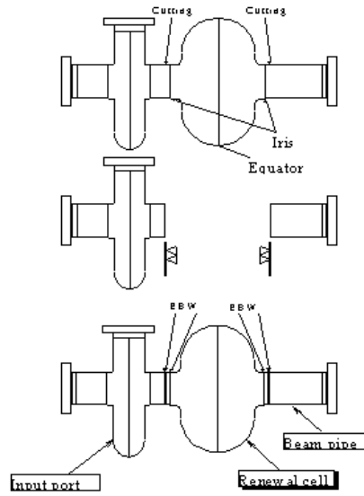
Fig.2 Removal processes of improper welded sections
