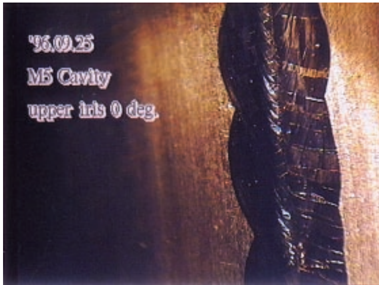
Fig.4 EBW seam in the M-5 Cavity
