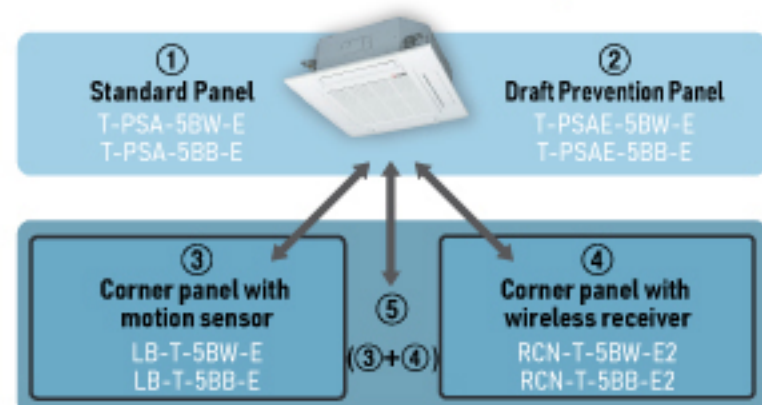
Installation position of Wireless kit and Motion sensor kit
