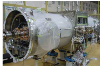
Figure 9: Cryomodule for c-ERL main linac
